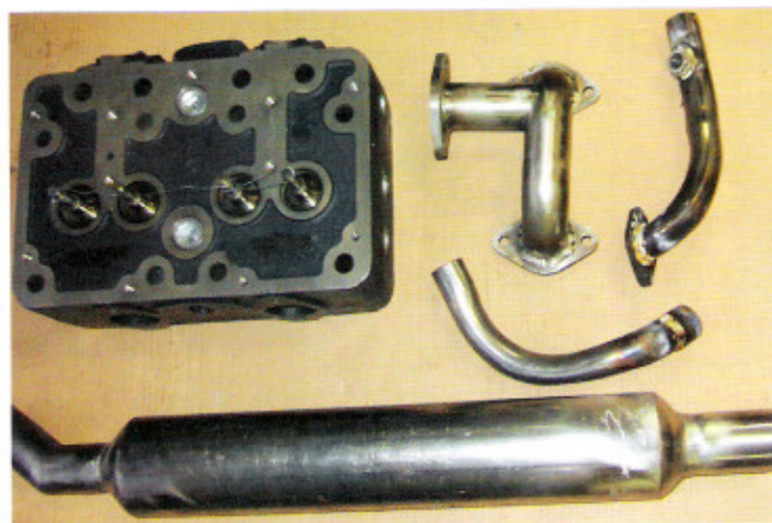
The Zetor 25 cylinder head, exhaust silencer, exhaust flange and water pump pipes seen here are all available from Moto-Check.
