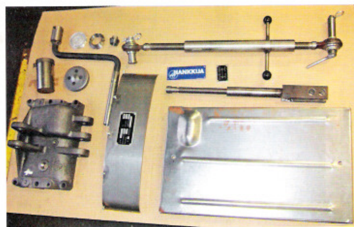
Another group of Zetor components available from Moto-Check include a hydraulic lift cover, battery box cover, filler cap, pto shaft guard, factory emblem, gearing diagram, oil plug, upper link, starting crank, right-hand strut and strut screw.
